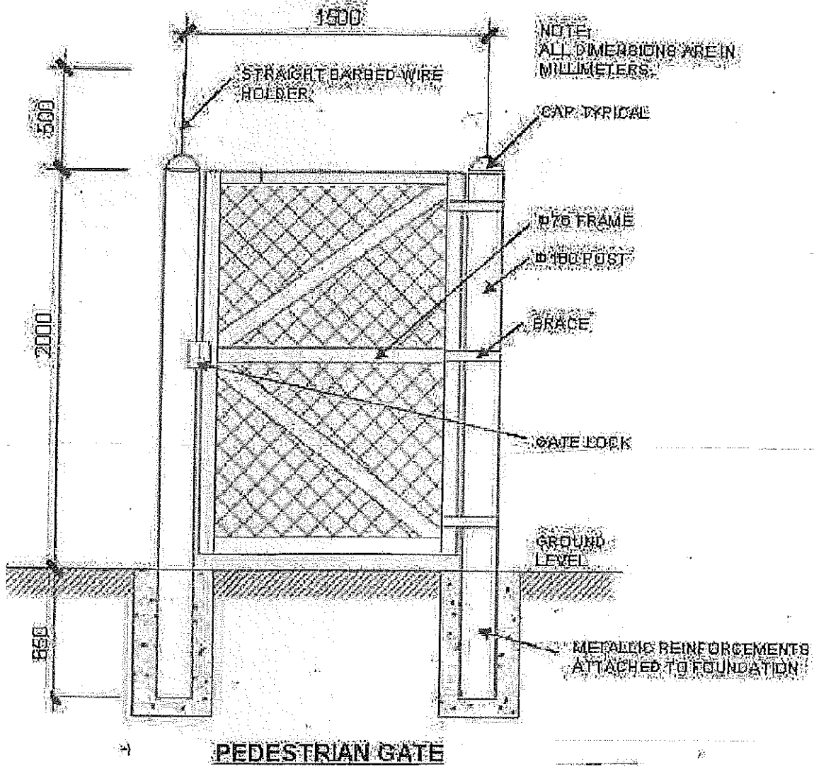
DRAWING OF PEDESTRIAN GATE
